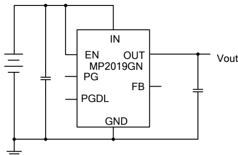
Output-Fixed Version
